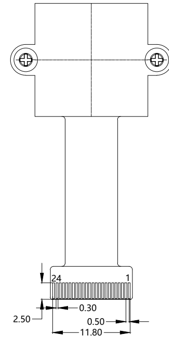
BOTTOM VIEW
